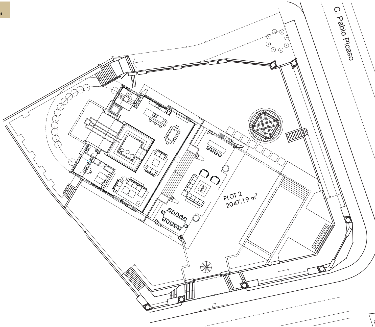
SITE PLAN ▶
