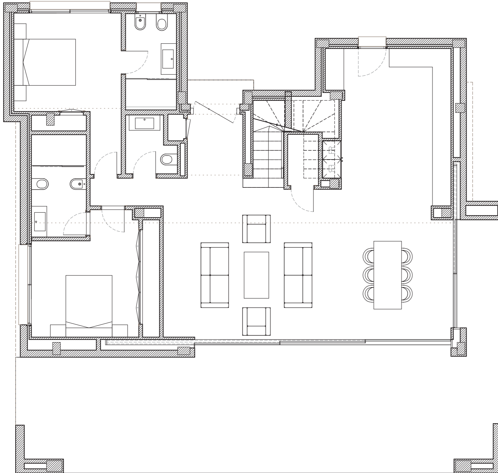
GROUND FLOOR
